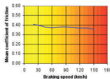
E 368 Friction values with speed
