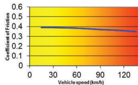
E400 nominal friction level
