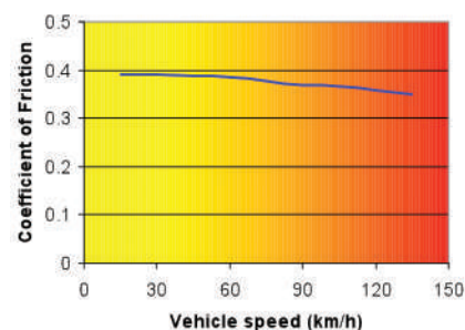
E 308 Friction values with speed
