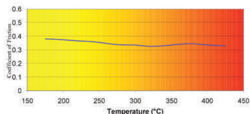
E 352A Friction values with Temperature
