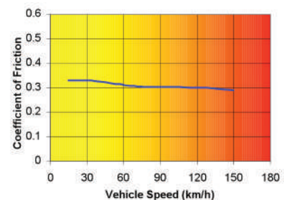
E 349 Friction values with speed
