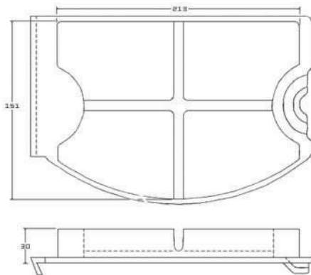
Integral Clip Pad Left Hand
