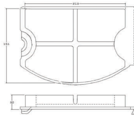
Integral Clip Pad Right Hand
