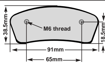
FA509A Thickness: 13mm Type: Tony Kart
