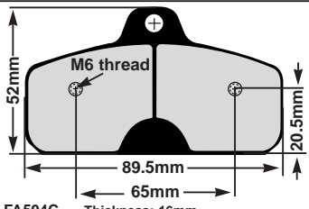
FA504C Thickness: 16mm Type: Birel (Italy)/ Kestrel (Italy)/ Blesse (Italy) 100cc/ 125cc Rear
