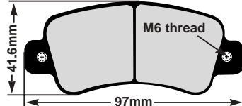
FA503 Thickness: 11mm Type: Hekakart FA503A Thickness: 14.5mm Type: Kartsport (Boxer) (Will also fit Zip Pro-Kart) Kart Pro - Stratos
