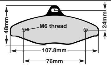
FA510 Thickness: 14mm Type: CRG (Italy)
