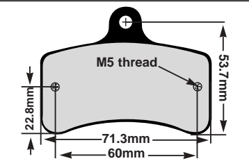
FA507 Thickness: 16mm Type: Tony Kart (rear)
