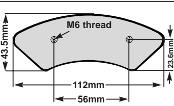
FA511 Thickness: 14mm Type: Swiss Hutless
