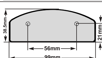
FA517 Thickness: 17.3mm Type: Techno-Kart (rear)
