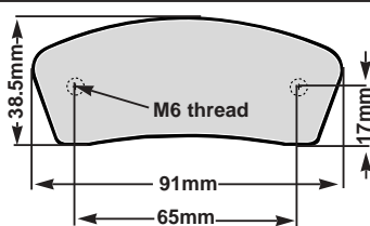
FA509B Thickness: 13mm Type: Tony Kart All Kart
