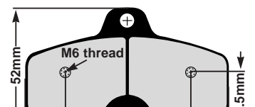
FA504B Thickness: 11.5mm Type: Birel (Italy)
