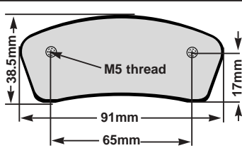
FA509 Thickness: 13mm Type: Tony Kart
