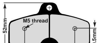
FA504 Thickness: 16mm Type: Haase/Tony Kart/Tibikart
