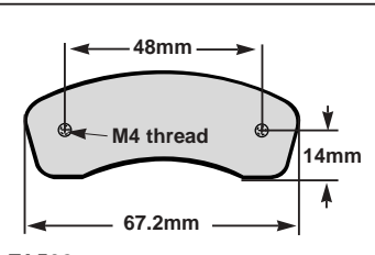
FA502 Thickness: 7.3mm Type: Tony Kart (rear)
