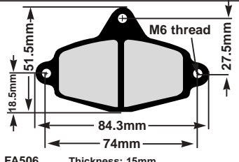
FA506 Thickness: 15mm Type: CRG (Italy)/ TKM (UK) (Tal - Ko 100cc)
