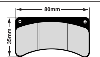
FA515 Thickness: 9mm Type: Kelgate (6 piston) Also used on Anderson Karts)
