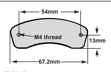
FA502B Thickness: 7.3mm Type:
