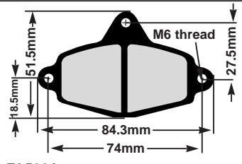
FA506A Thickness: 10.2mm Type: CRG (Italy)
