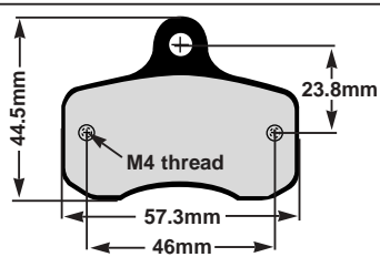
FA501 Thickness: 10mm Type: Tony Kart (front)
