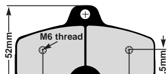
FA504A Thickness: 13mm Type: Righetti Ridolfi
